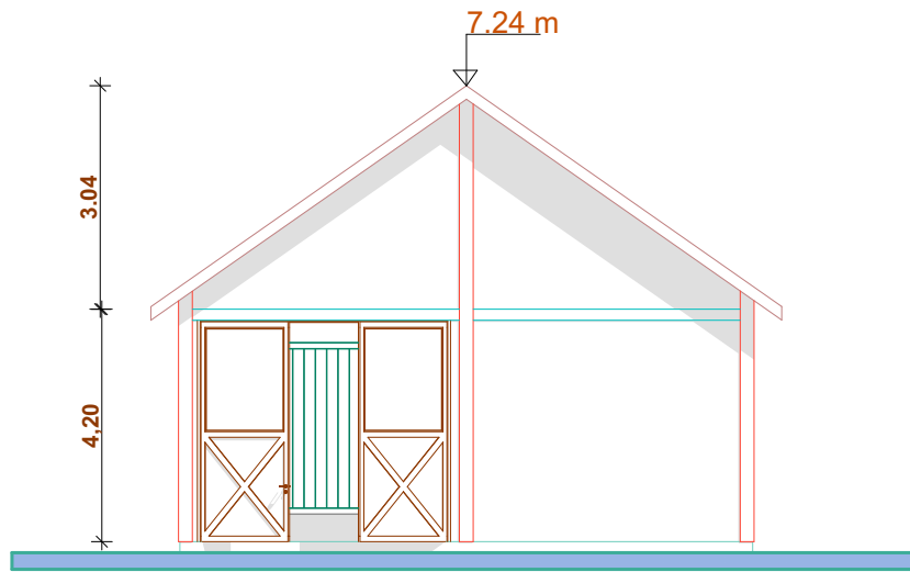
Façade principale
